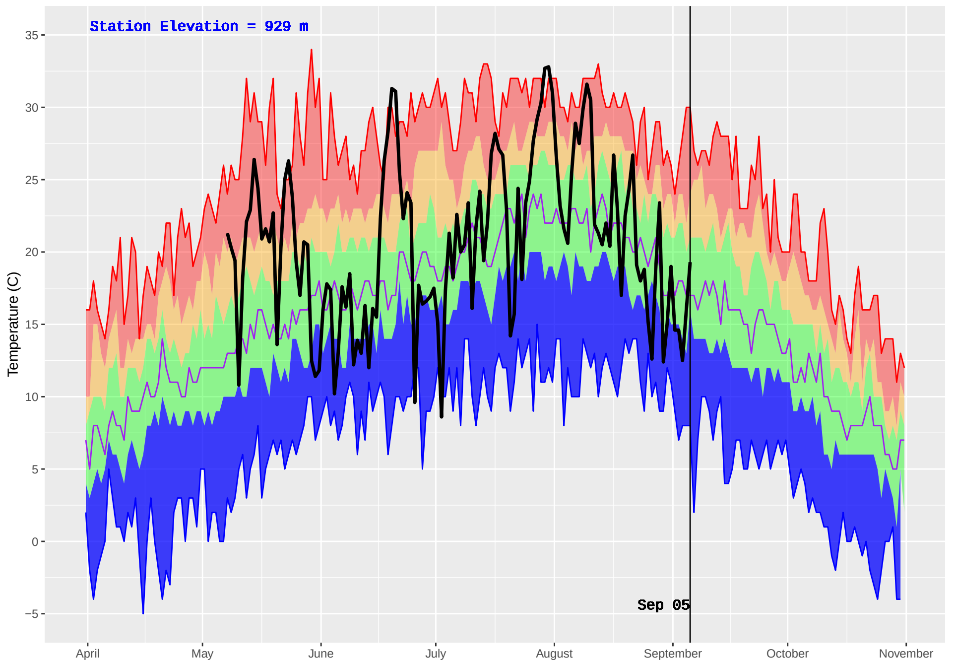
RISKE CREEK (210) : Historical (1980–2016) and Current (2018) Daily Temperature
