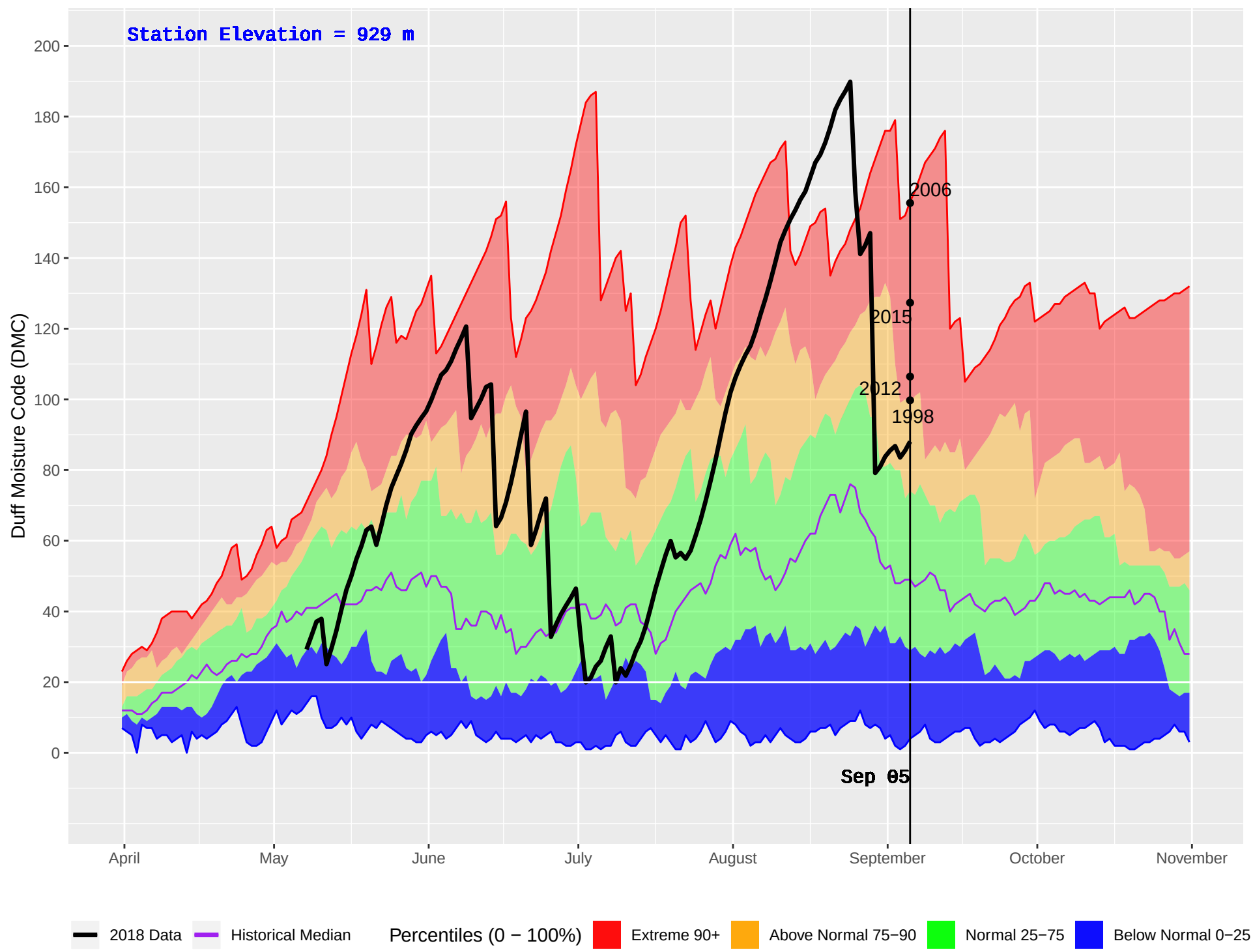
RISKE CREEK (210) : Historical (1980–2016) and Current (2018) Daily Duff Moisture Code (DMC)
